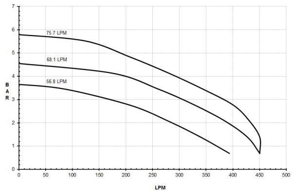
9303C-HM4C-SP & 9303S-HM4C-SP METRIC
