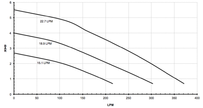
9303C-HM3C-SP & 9303S-HM3C-SP METRIC
