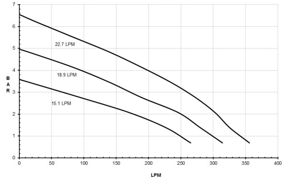
9303C-HM2C & 9303S-HM2C METRIC 9303C-HM2C-U & 9303S-HM2C-U
