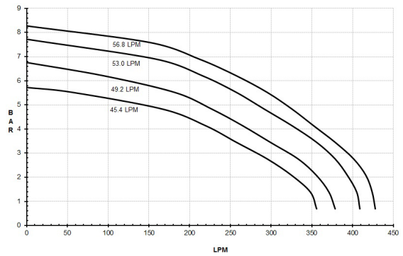
9303P-HM5C & 9303P-HM5C METRIC
