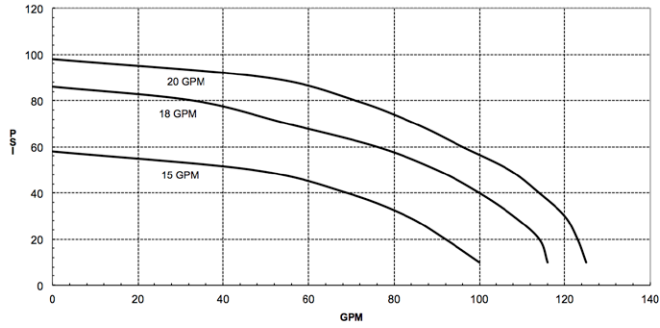
9303C-HM4C & 9303S-HM4C 9303C-HM4C-U & 9303S-HM4C-U
