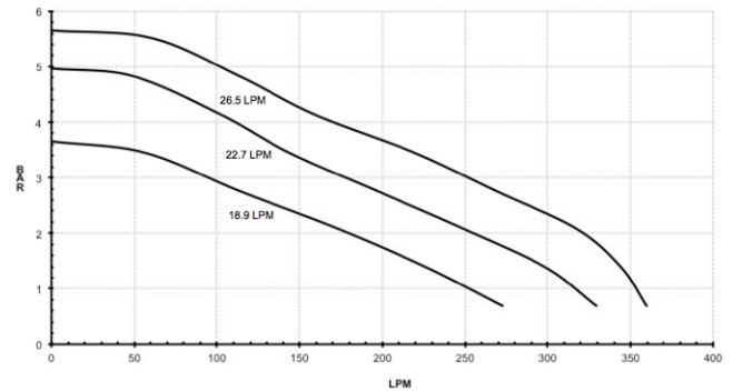
9303C-HM5C-SP & 9303S-HM5C METRIC-SP
